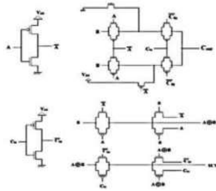
Figure 2: Full Adder Carry and Sum Generation
